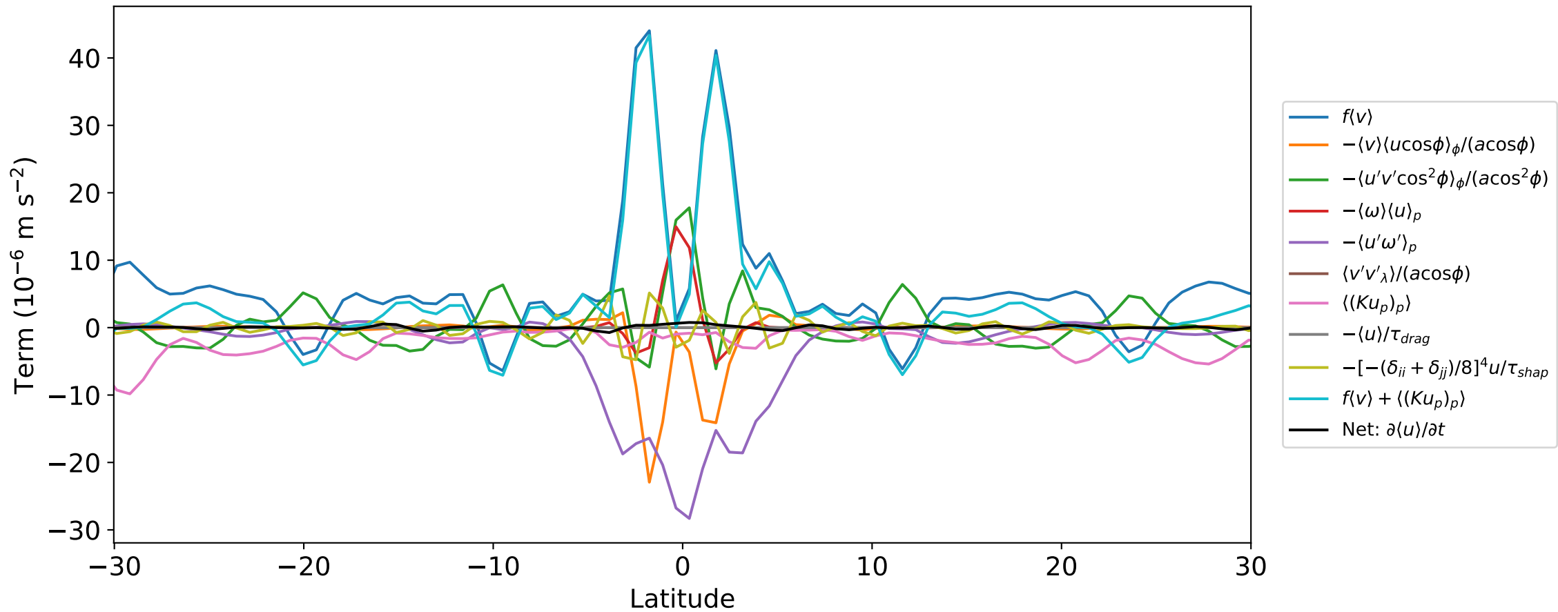
r112ct1 all terms, p = 0.40 bar, 100.00 day mean
